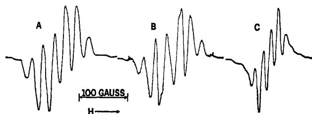
Figure 2. ESR spectra of (A) 4-methylheptane glass containing 1 mole % 1 I3MP photolyzed at 77°K for 44 min with the medium-pressure lamp, signal level 200; (B) 2-methylpentane glass containing 1 mole % 3 IMP photolyzed at 77°K for 1 hr with the medium-pressure lamp, signal level 320; (C) 3-chloro-3-methylpentane glass containing about 1 mole % naphthalene photolyzed at 77°K for 15 min with the high-pressure lamp filtered to remove wavelengths below 2800 Å, signal level 80.
